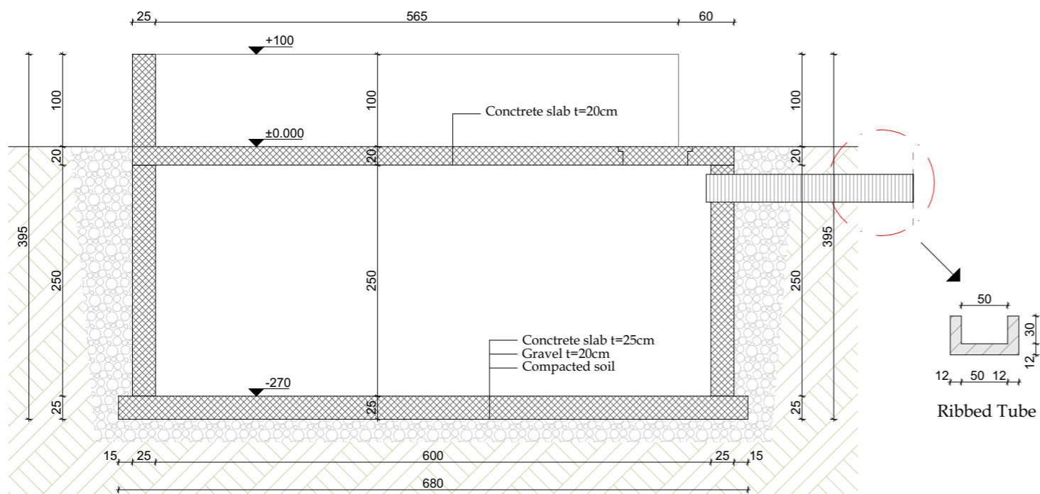
- SECTION 1-1
