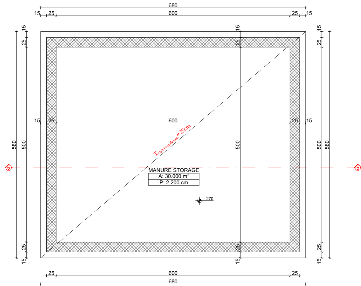
- FOUNDATION PLAN _ LEVEL - 270
