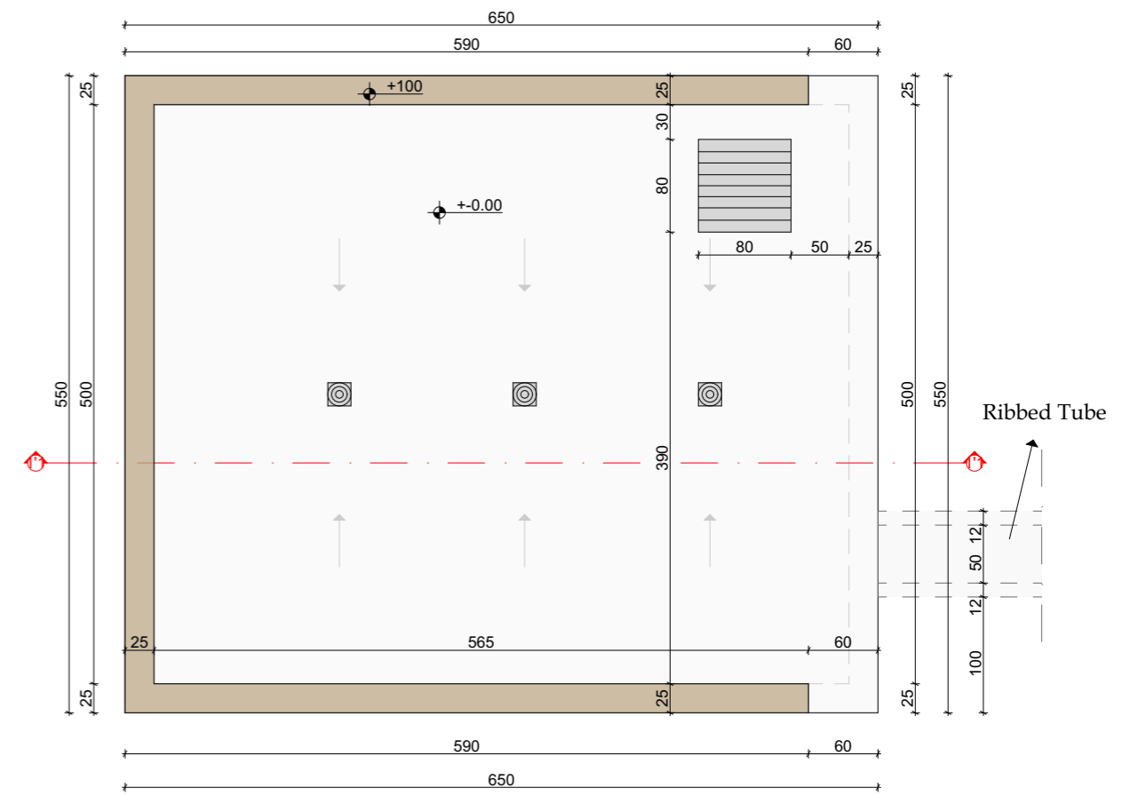
- BASE PLAN _ LEVEL +0.00
